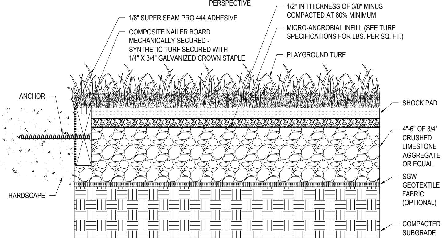
STANDARD INSTALL CROSS SECTION
